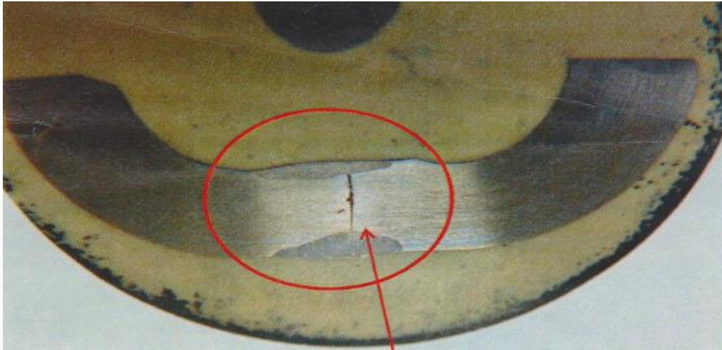
Figure A3 Showing a welding penetration defect of a chain link due to inadequate manufacturing processes.
